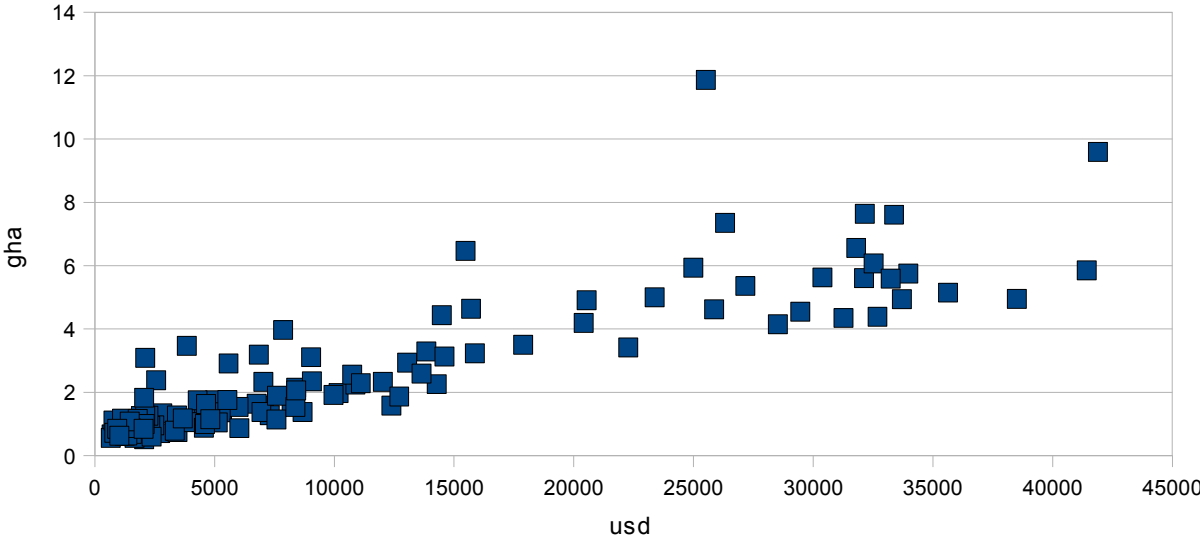
Figure 3: Per Capita Ecological Footprint and GDP of Countries (xy scatter plot)
